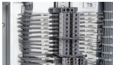
Wire ID and Terminal Block
